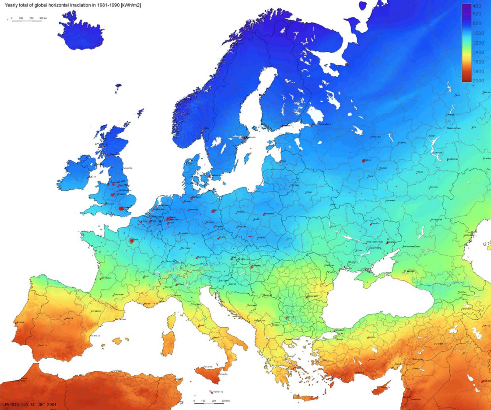
Yearly total of global horizontal irradiation in 1981-1990 [kWh/m 2 ]
