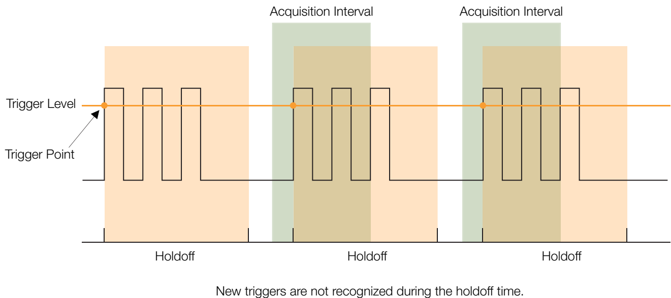
Figure 35. Trigger holdoff.
