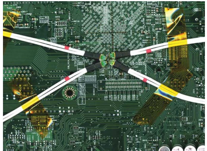
Figure 38. Dense devices and systems require small form factor probes.
