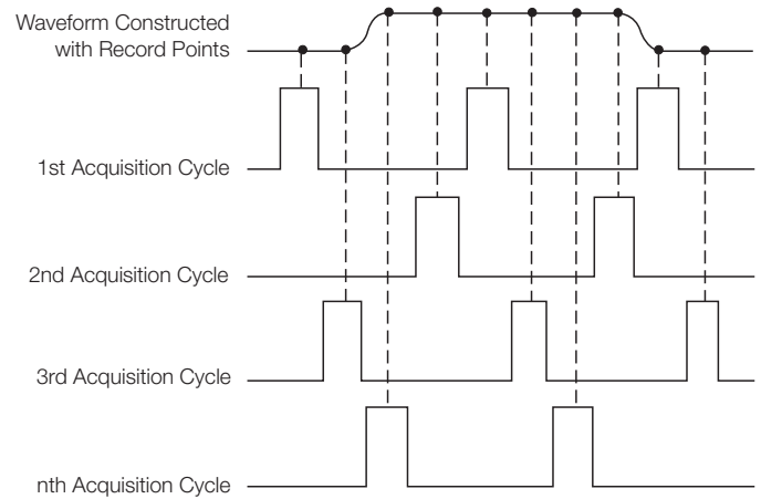
Figure 29. Some oscilloscopes use equivalent-time sampling to capture and display very fast, repetitive signals.
