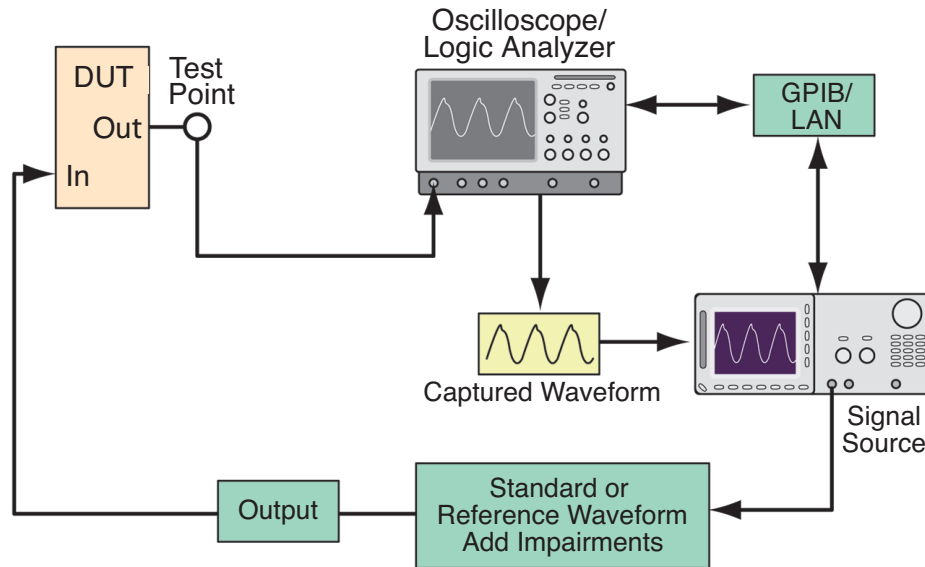
Figure 3. Signal generators can use standard, user-created or captured waveforms, adding impairments where necessary for special test applications.
