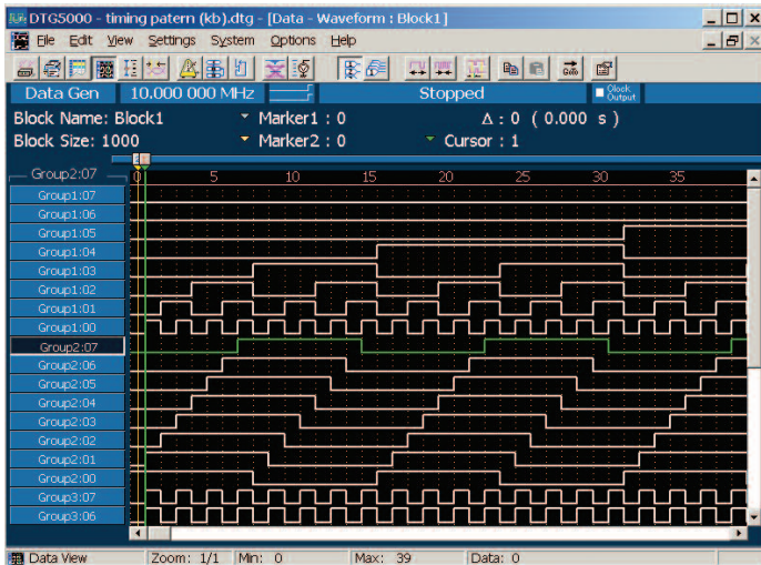
Figure 46. Multi-channel DTG s bus timing display.
