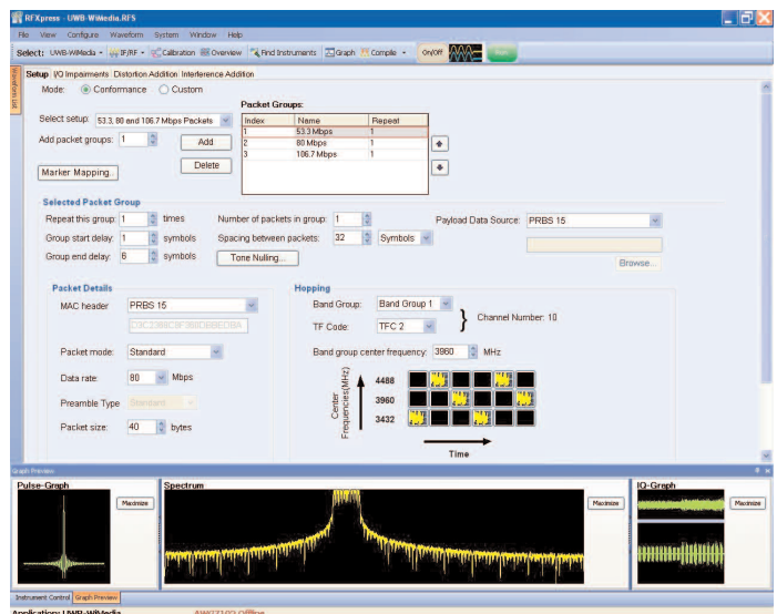
Figure 40. Complex UWB waveforms are easily created using RFXpress.
