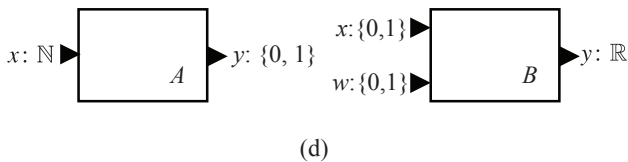
Figure 13.6: Four pairs of actors whose type refinement relationships are explored in Exercise 1.
