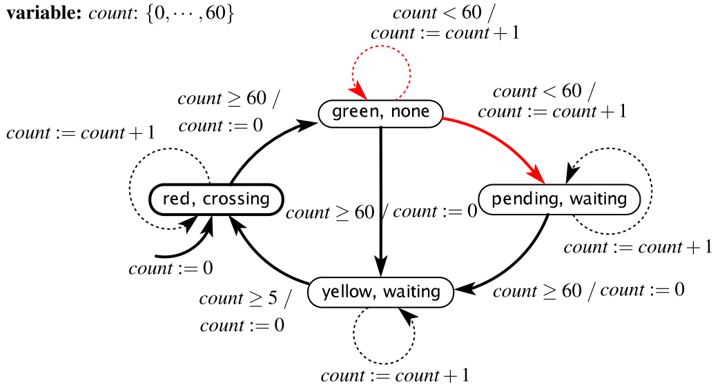
Figure 14.4: Extended state machine obtained from synchronous-reactive composition of traffic light controller and pedestrian models. Note that this is non-deterministic.
