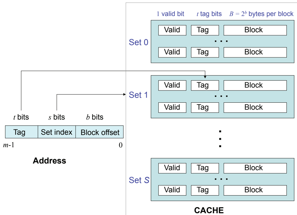
Figure 8.2: Cache Organization and Address Format. A cache can be viewed as an array of sets, where each set comprises of one or more cache lines. Each cache line includes a valid bit, tag bits, and a cache block.
